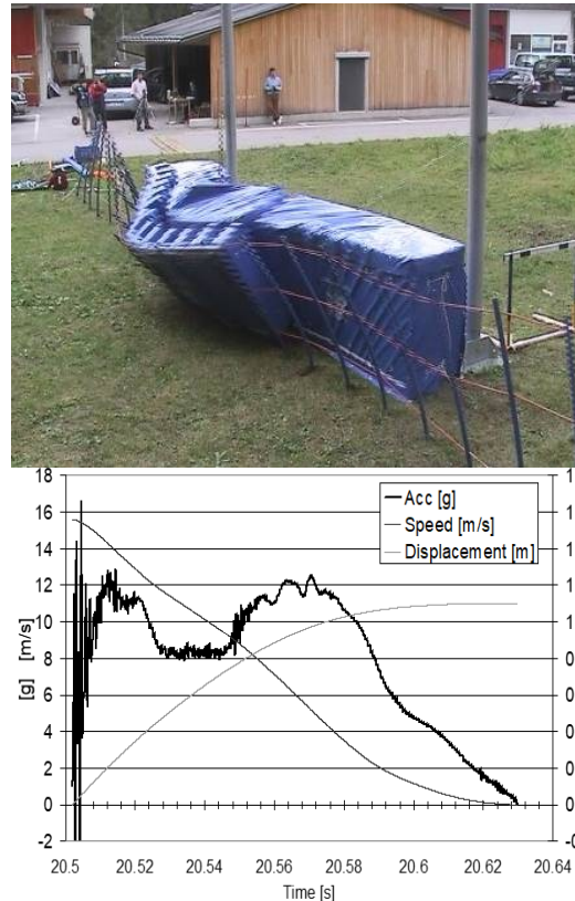
Outdoor test with Pendulum and instrumented dummy.
